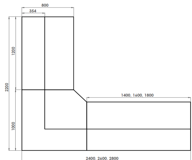
Low Corner, High Corner, High Corner with Glass & High Corner with DDA module
