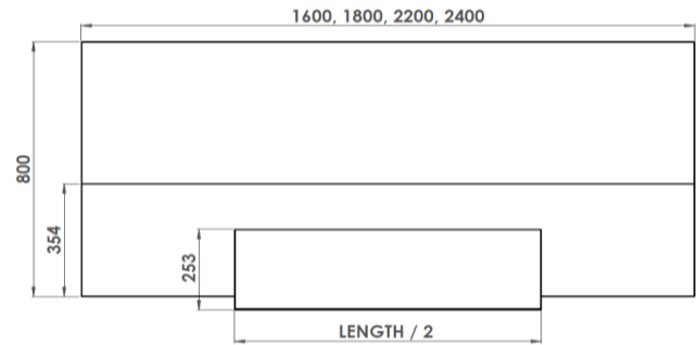
Low Straight & High Straight with Feature Front Layout
