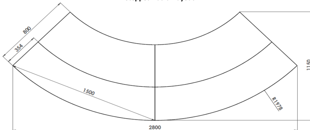
Low Radial, High Radial, High Radial with Glass & Stepped Radial Layout
