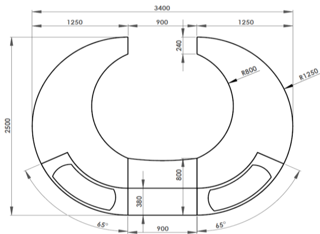
Double High Extended Reception
