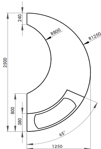
Single High Extended Reception
