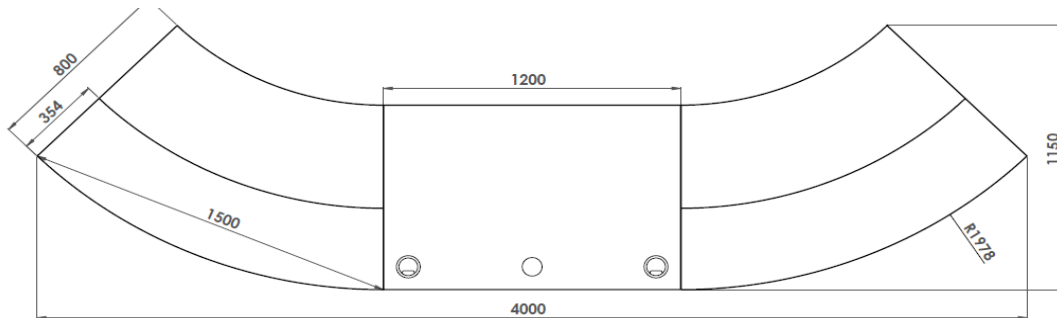
Low Quadrant, High Quadrant, High Quadrant with Glass & High Quadrant with DDA module layout
