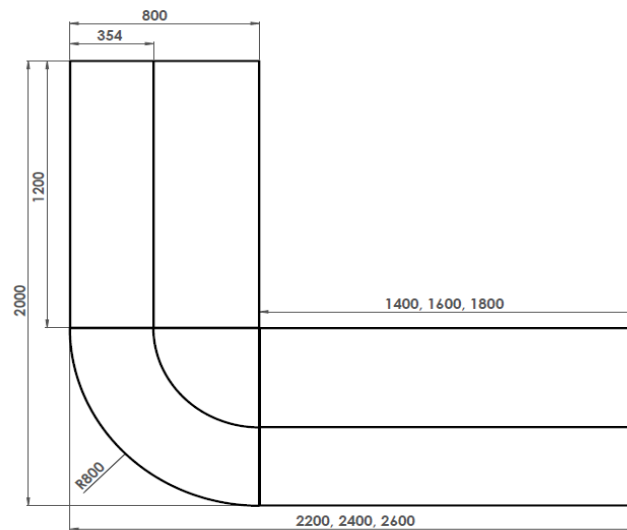
Low Annular, High Annular, High Annular with Glass & High Annular with DDA module layout
