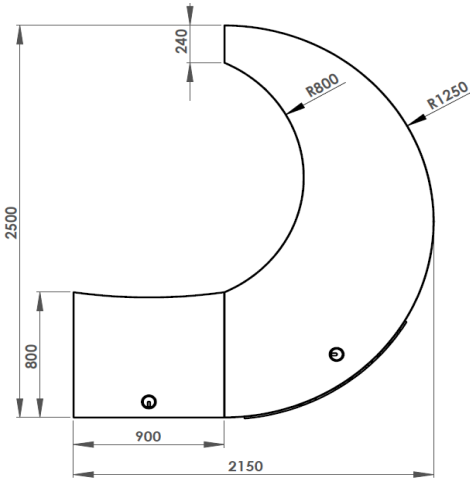
Single Low Extended & Single Low Extended Screen Reception
