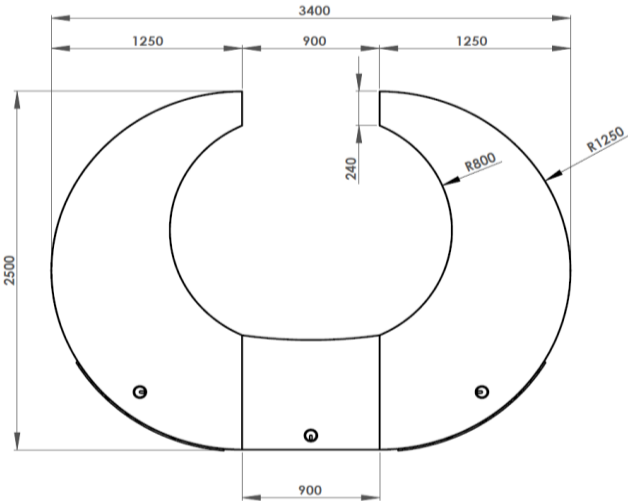
Double Low Extended & Double Low Extended Screen Reception
