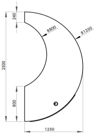
Single Low & Single Low with Screen Reception
