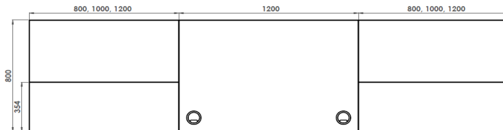
High Extended Straight, High Extended Straight with Glass & High Extended Straight with DDA module layout
